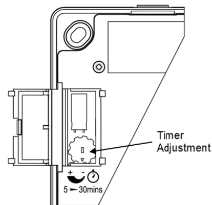
FIG. 5: PIR TIMER
